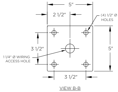
Luminaire Mounting Plate
