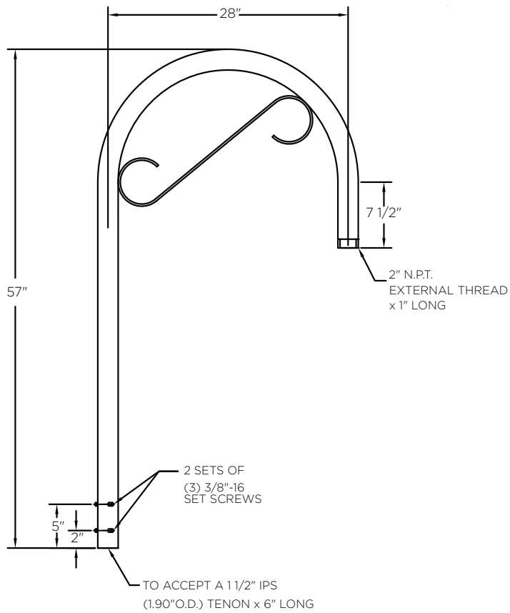
Tenon Mount Single Arm
