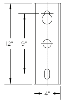
Side Mount Details 4" x 1 3/4" x 12"L
